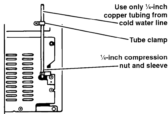
Style #2 valve
