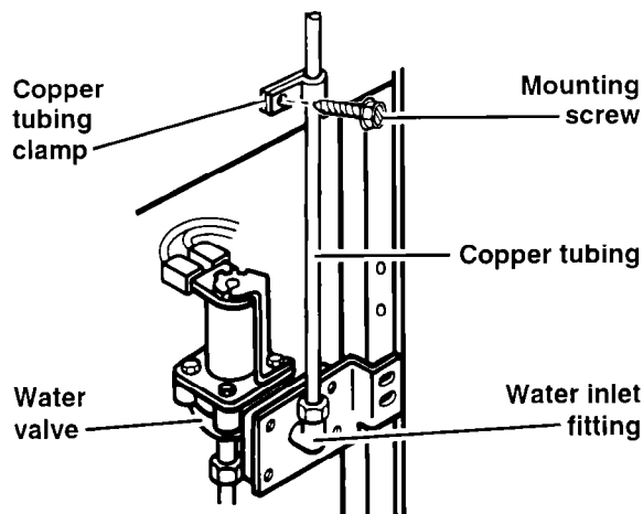
Style #1 valve
